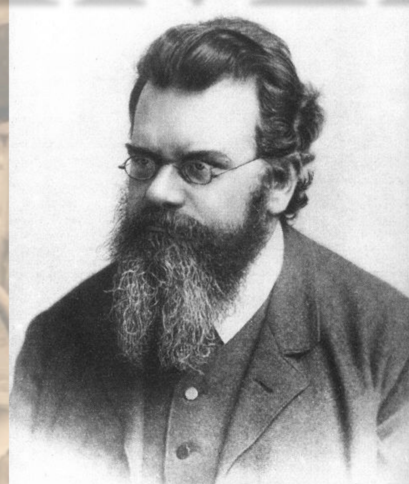
Ludwig Boltzmann 1844-1906
