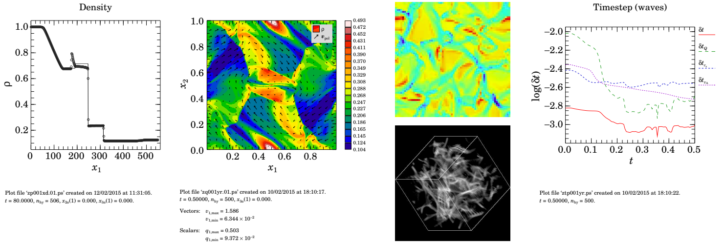
Figure 3: From left to right: 1-D line (bubble) plot of the density in the Brio & Wu shock tube problem; a colour contour plot showing both density and velocity vectors from the Orszag-Tang vortex; a 2-D pixel plot of the velocity divergence (top) and a line-of-sight integration dump of the synchrotron emissivity in a low resolution ( 64^3 ) run of super-Alfvénic turbulence; and a time slice plot showing how the time-steps, \delta t , evolve over the course of a simulation.
